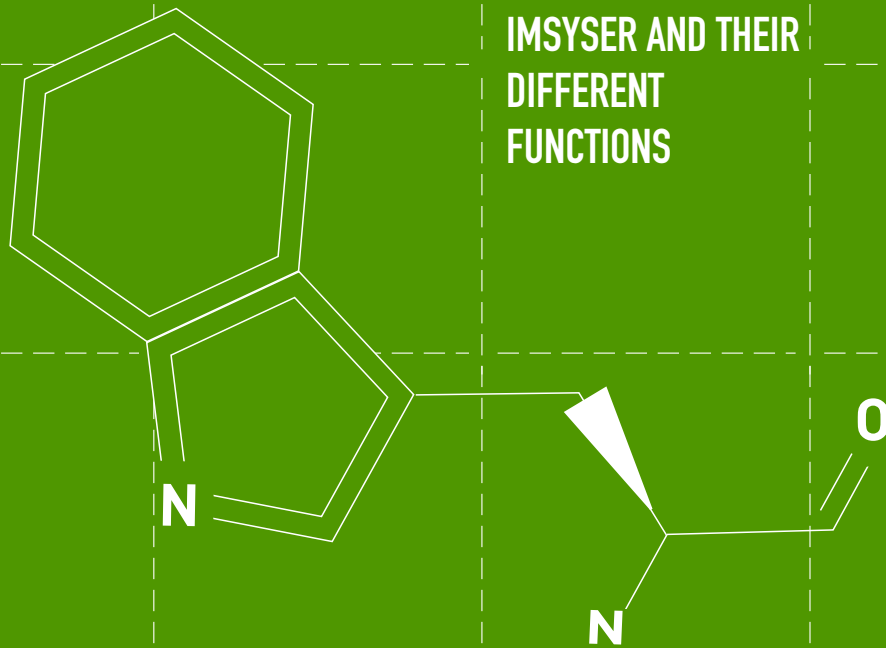
fig 1 tryptophan
